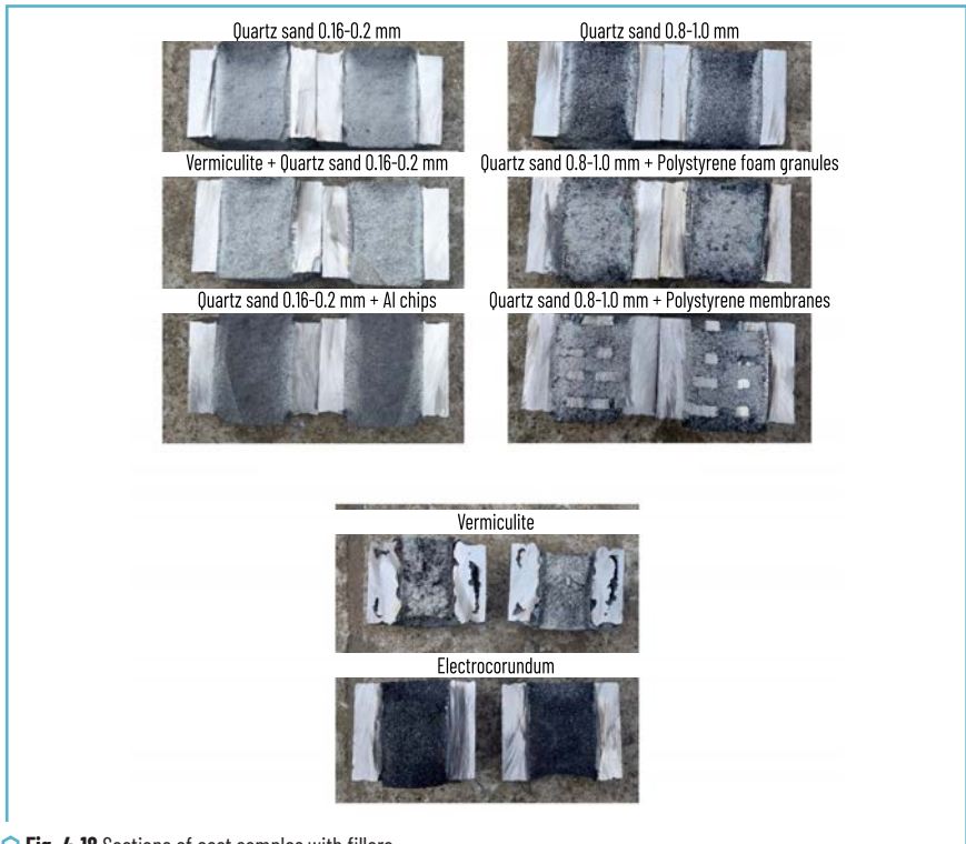
Fig. 4.18 Sections of cast samples with fillers
