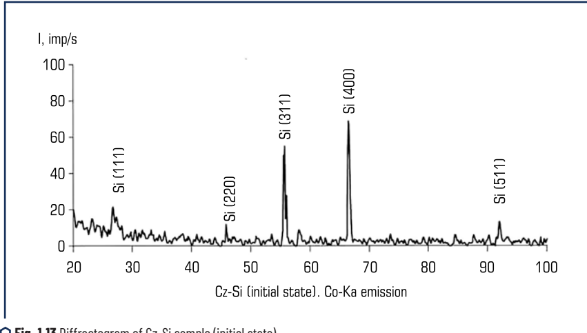
○ Fig. 1.13 Diffractogram of Cz-Si sample (initial state) Source: [44]
