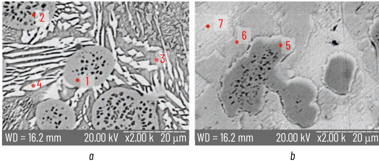
○ Fig. 3.3 Microstructures of cast high-entropy alloys: a – No. 4 and b – No. 5 of the FeNiCrCuAl and FeNiCrCuMn systems. Individual phases are indicated by numbers, and their chemical composition is given in Table 3.3
