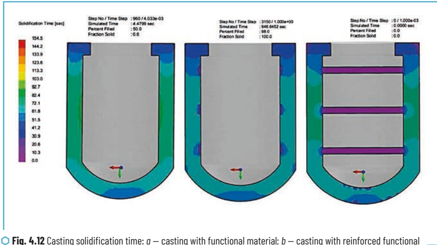
Fig. 4.12 Casting solidification time: a – casting with functional material; b – casting with reinforced functional material; c – casting with functional filler, which is reinforced from the liquid phase of the shell metal
