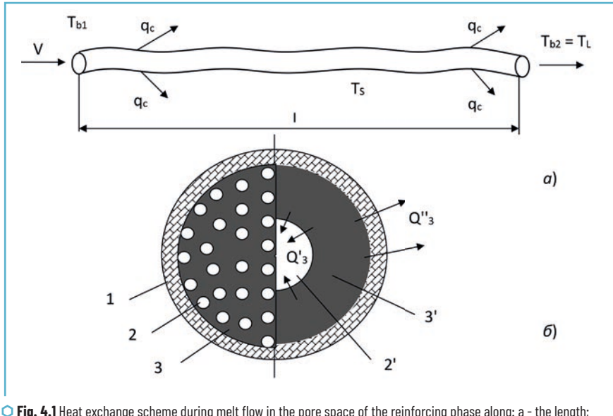
Fig. 4.1 Heat exchange scheme during melt flow in the pore space of the reinforcing phase along: a - the length; b - the cross-section of the mold with RE oriented in it: (b); 1 – shell (mold); 2 – reinforcing element; 3 – matrix melt; 2' – equivalent cross-section of the reinforcing element; 3' – equivalent cross-section of the matrix melt Source: [3]
