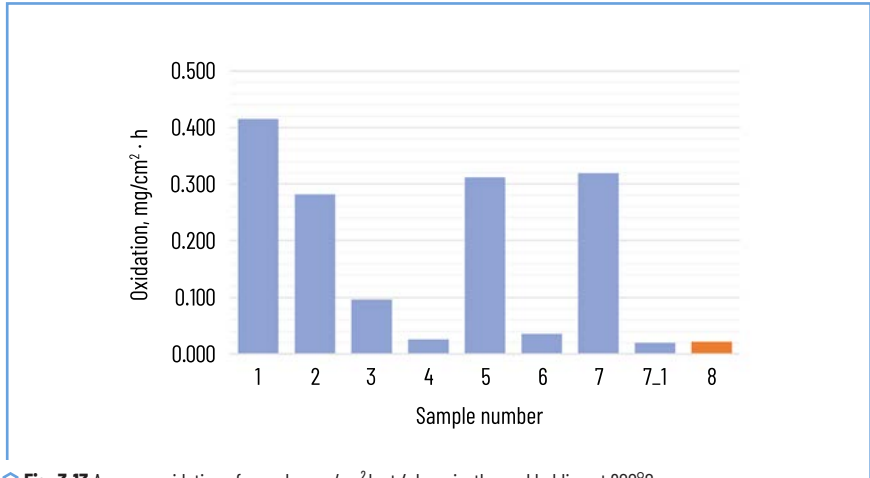
Fig. 3.13 Average oxidation of samples mg/cm 2 ·h at 4-hour isothermal holding at 900°C
