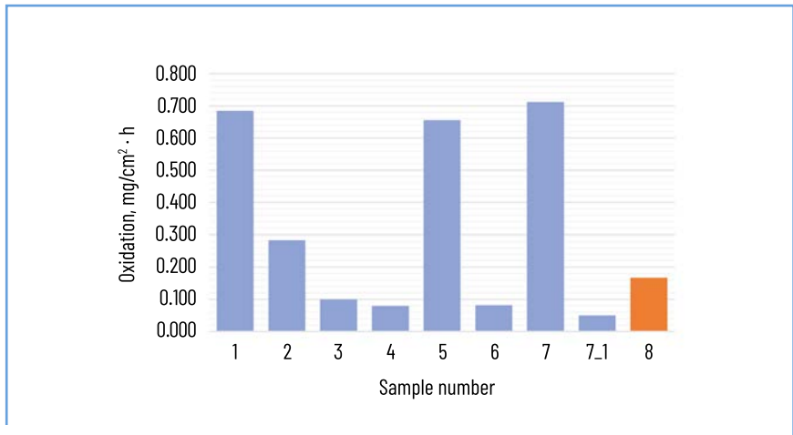
Fig. 3.14 Average oxidation of samples mg/cm 2 ·h at 4-hour isothermal holding at 1000°C
