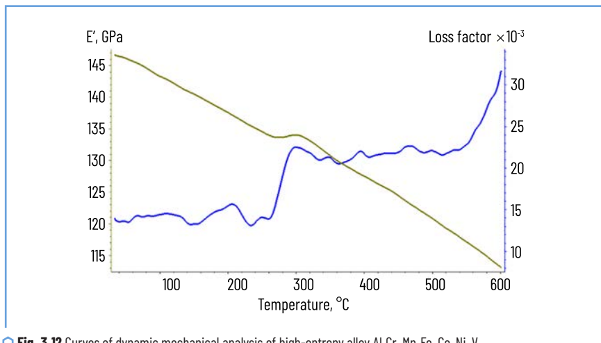
Fig. 3.12 Curves of dynamic mechanical analysis of high-entropy alloy \text{Al}_5\text{Cr}_{15}\text{Mn}_{11}\text{Fe}_{18}\text{Co}_{17}\text{Ni}_{31}\text{V}_3
