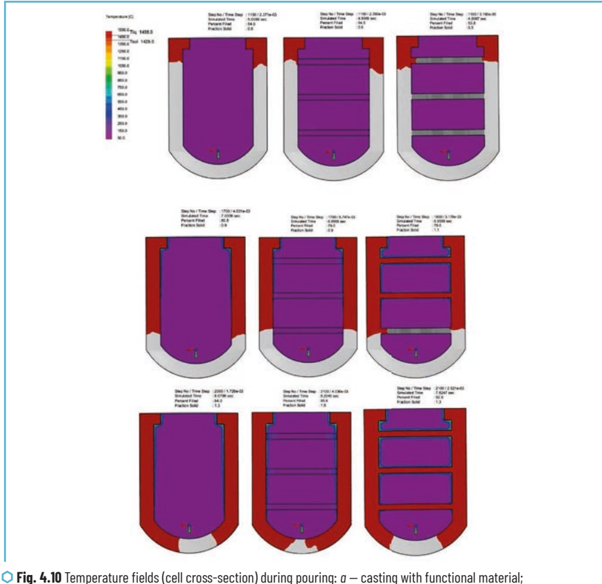
⊙ Fig. 4.10 Temperature fields (cell cross-section) during pouring: a – casting with functional material; b – casting with reinforced filler; c – casting with functional filler reinforced from the liquid phase of the shell metal
