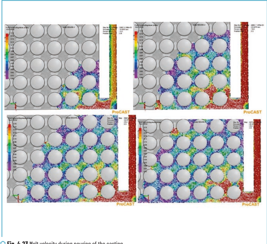
○ Fig. 4.23 Melt velocity during pouring of the casting
