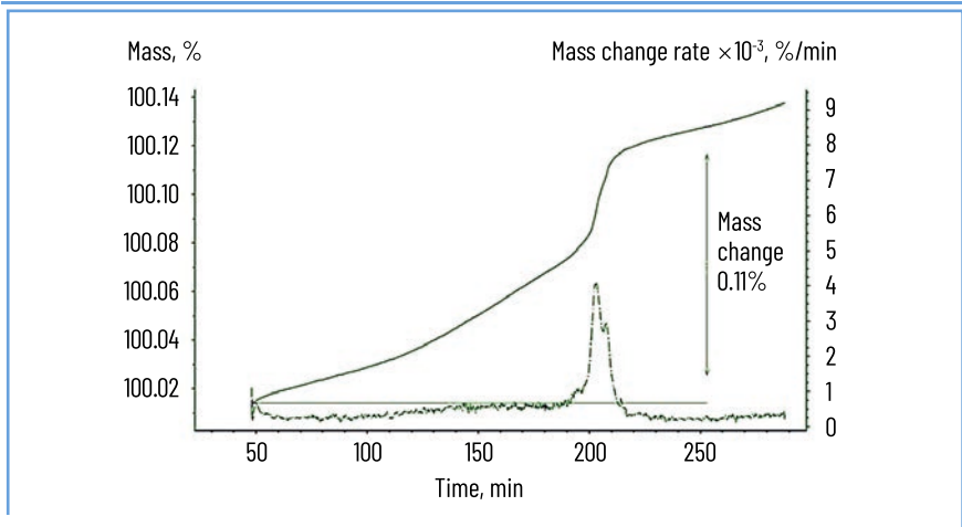
Fig. 3.15 Thermogravimetric diagram of steel GX10CrNiMn18-9-1 when exposed to artificial air at 1000°C
