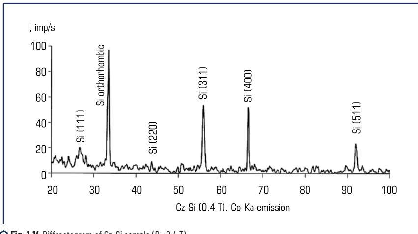
○ Fig. 1.14 Diffractogram of Cz-Si sample ( B=0.4 T) Source: [44]
