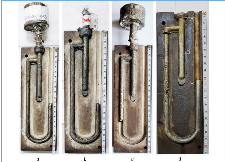
○ Fig. 3.5 Filled U-shaped channels in the Nehendzi–Kuptsov test mold with overfills for determining the fluidity of various alloys: a – casting from stainless steel GX10CrNiMn18-9-1 ( \lambda = 262 mm); b – steel casting G25 ( \lambda = 277 mm); c – high-entropy alloy casting of the FeNiCrCuMn system ( \lambda = 142 mm); d – high-entropy alloy casting of the FeNiCrCuAl system ( \lambda = 320 mm)
