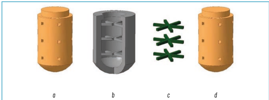
Fig. 4.6 General view of 3D models: a – cell; b – cell with membranes; c – reinforcement, d – core with channels
