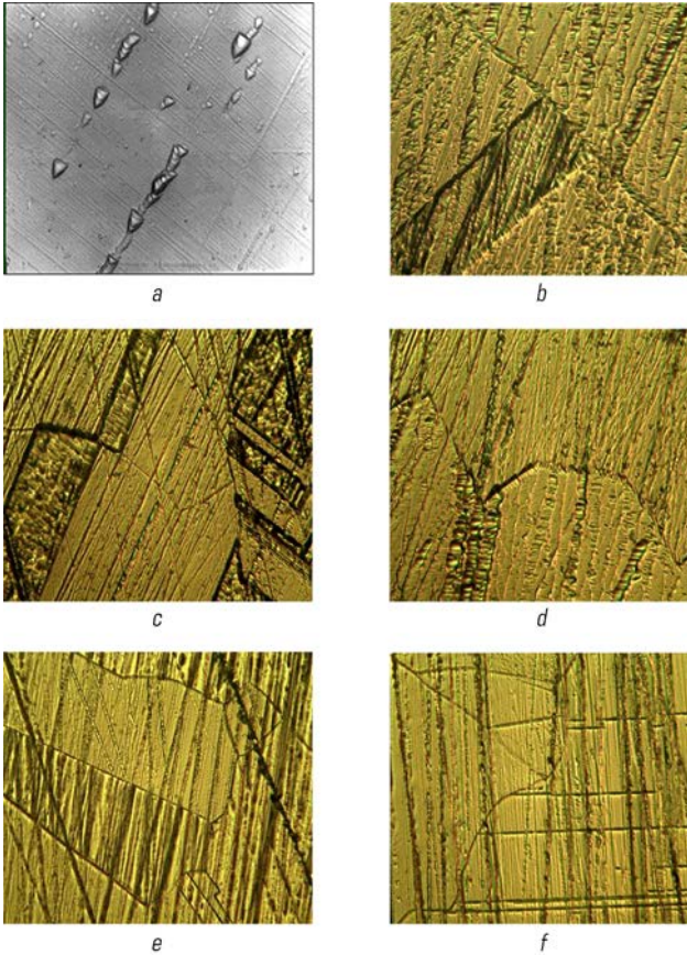
○ Fig. 1.6 Microstructures of Cz-Si samples: a - initial state, \times 500 ; b, c, d - after 240 hours of exposing to direct-current magnetic field, \times 400 ; e, f - after 720 hours of exposing to direct-current magnetic field, \times 400
