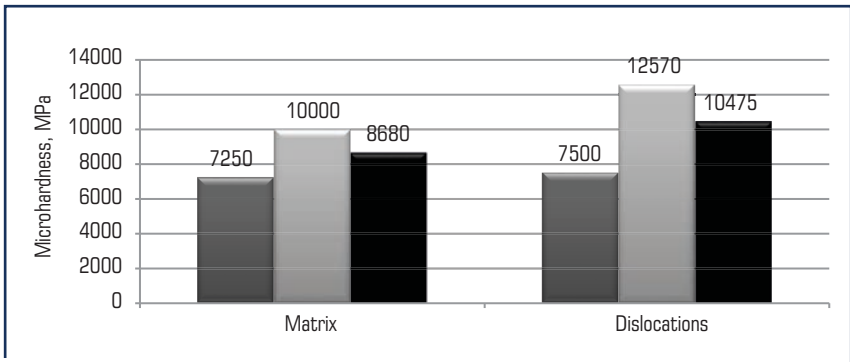
Fig. 1.28 Microhardness per the structural units of Cz-Si(Zr) samples (in the initial state, after 240 hours and 720 hours of exposing to direct-current magnetic field)
