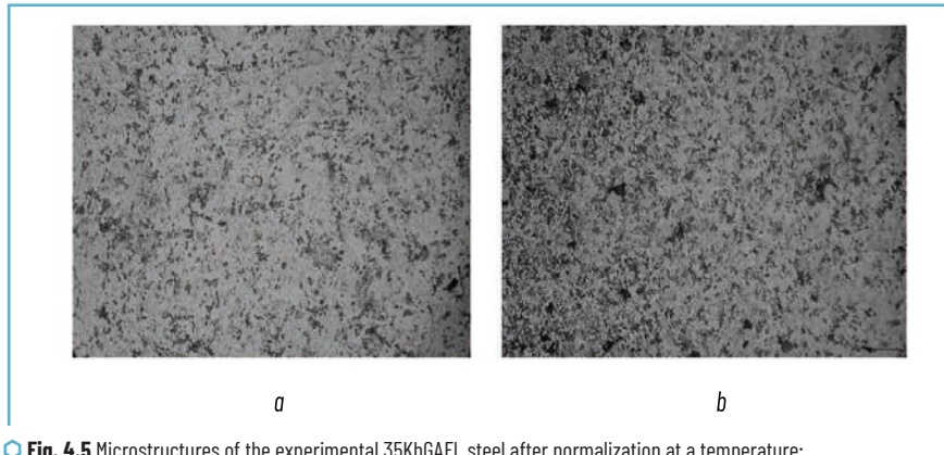
○ Fig. 4.5 Microstructures of the experimental 35KhGAFL steel after normalization at a temperature: a – of 930°C; b – normalization at a temperature of 930°C + tempering at a temperature of 510°C; ×200
