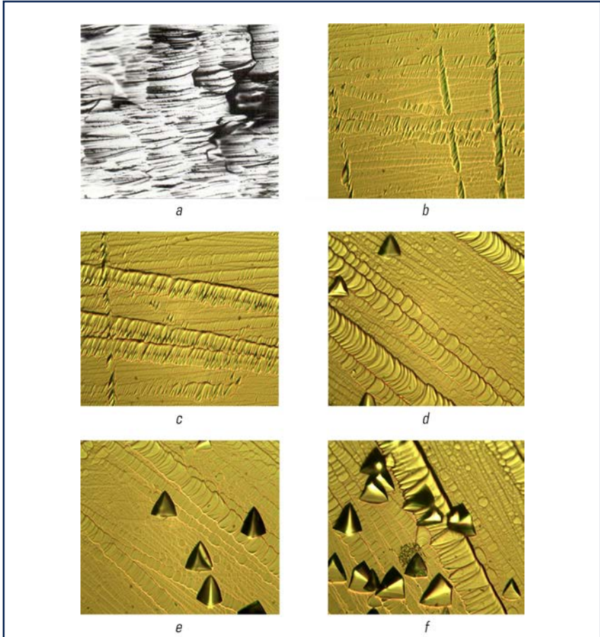
Fig. 1.11 Microstructures of Cz-Si samples doped with Mg: a – initial state, \times 1000 ; b – after 240 hours of exposing to direct-current magnetic field, \times 400 ; c, d – after 720 hours of exposing to direct-current magnetic field, \times 400 Source: [33–36]
