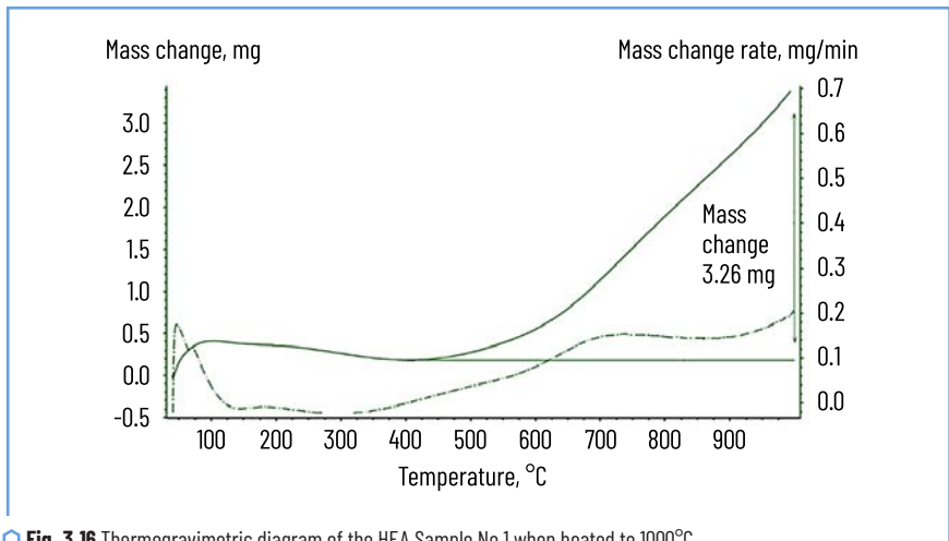
Fig. 3.16 Thermogravimetric diagram of the HEA Sample No.1 when heated to 1000°C
