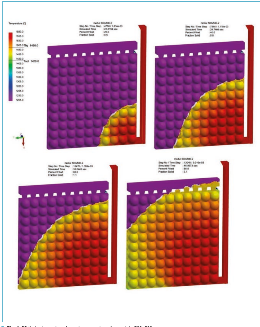
Fig. 4.22 Hydrodynamics of pouring a casting of a module 500x500
