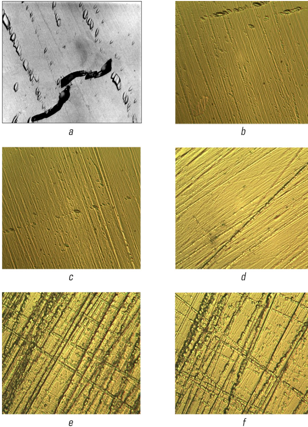
Fig. 1.8 Microstructures of Cz-Si samples doped with Cu: a – initial state, \times 500 ; b , c – after 240 hours of exposing to direct-current magnetic field, \times 400 ; d – after 720 hours of exposing to direct-current magnetic field (sample No. 1), \times 400 ; e , f – after 720 hours of exposing to direct-current magnetic field (sample No. 2), \times 400 Source: [33–36]
