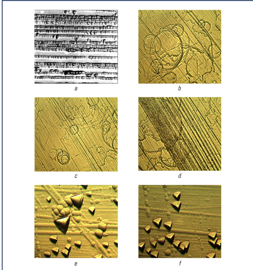
◉ Fig. 1.10 Microstructures of Cz-Si samples doped with Hf: a – initial state, \times 500 ; b, c, d – after 240 hours of exposing to direct-current magnetic field, \times 400 ; e, f – after 720 hours of exposing to direct-current magnetic field, \times 400 Source: [33–36]
