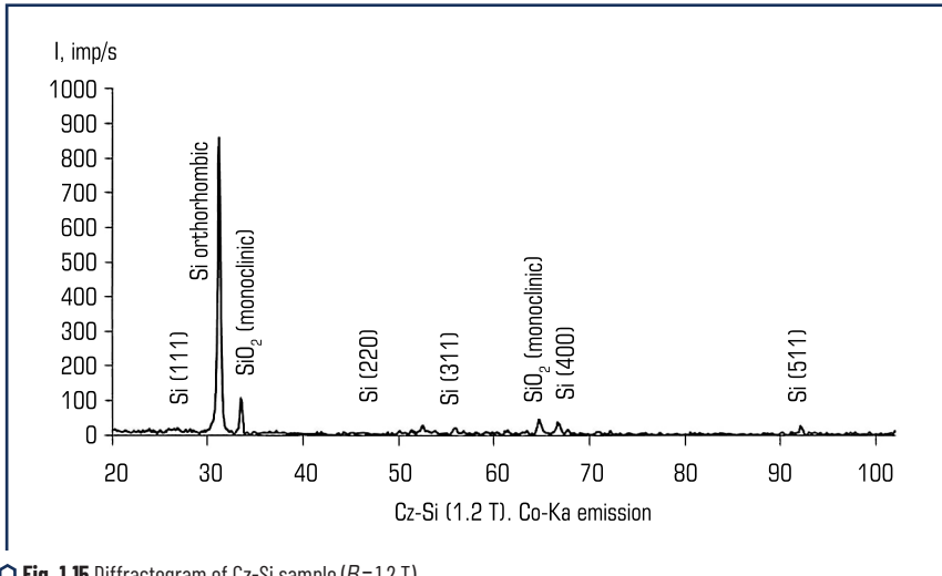
Fig. 1.15 Diffractogram of Cz-Si sample ( B=1.2\text{ T} ) Source: [44]
