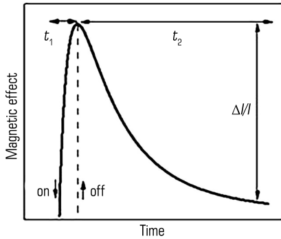
◻ Fig. 1.1 Dependence diagram between a gradual change in the crystal physical properties within a magnetic field (with a time constant t_1 ) and a relaxation after the magnetic field removal (with a time constant t_2 ); a relative change in a physical value of D/I is marked with a vertical arrow Source: [27]
