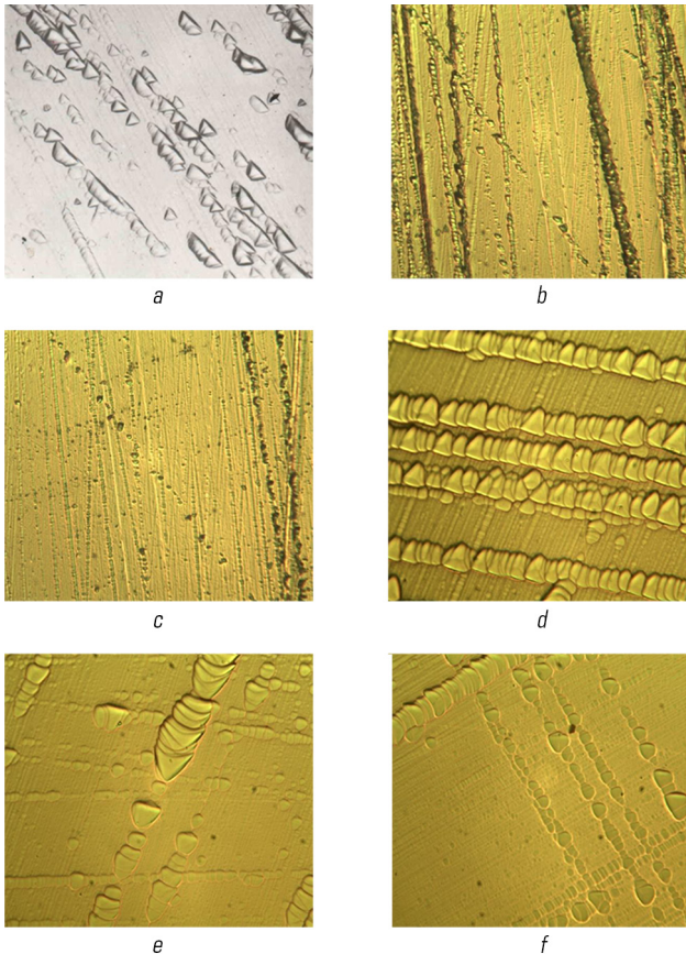
○ Fig. 1.12 Microstructures of Cz-Si samples doped with Fe: a – initial state, \times 500 ; b , c – after 240 hours of exposing to direct-current magnetic field, \times 400 ; d , e , f – after 720 hours of exposing to direct-current magnetic field, \times 400
