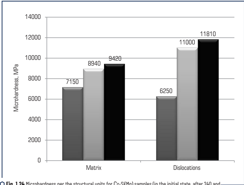
Fig. 1.24 Microhardness per the structural units for Cz-Si(Mg) samples (in the initial state, after 240 and 720 hours of exposing to direct-current magnetic field)
