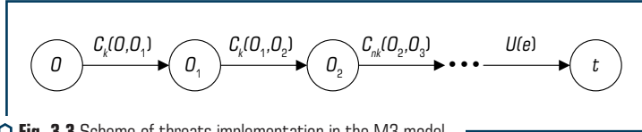
Fig. 3.3 Scheme of threats implementation in the M3 model
